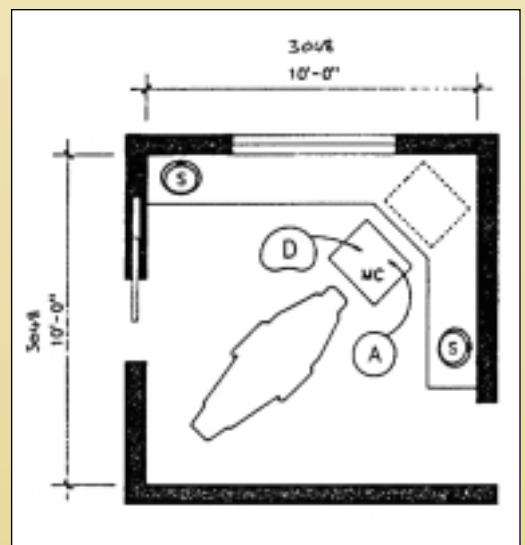
Figure 2: L-shaped set-up
